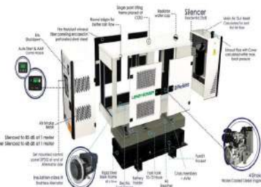
ATP ENCLOSURE/CANOPY
